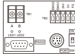
IAI's SIO converter "RCB-TU-SIO-A/B"
