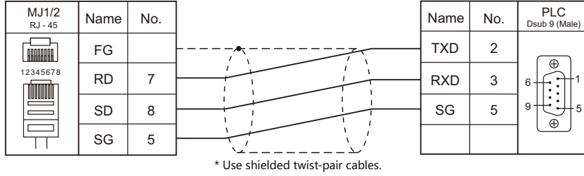
Wiring diagram 1 - M2
