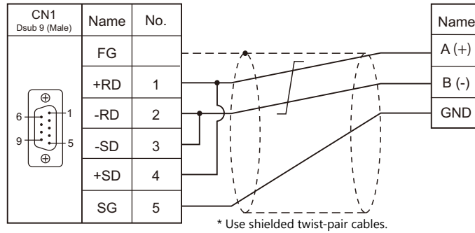
Wiring diagram 1 - C4
