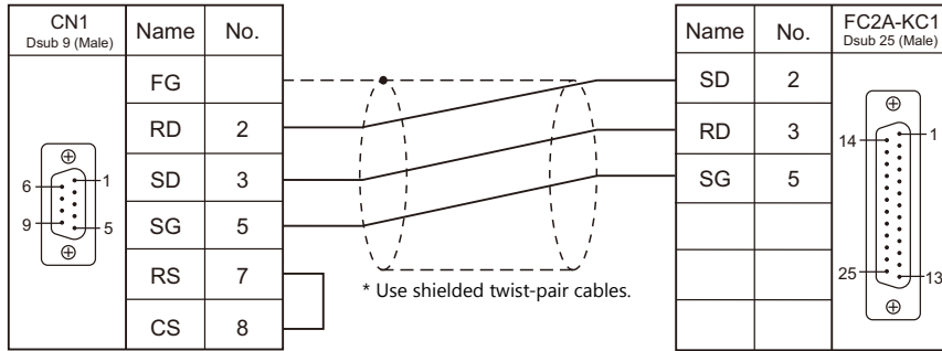
Wiring diagram 2 - C2
