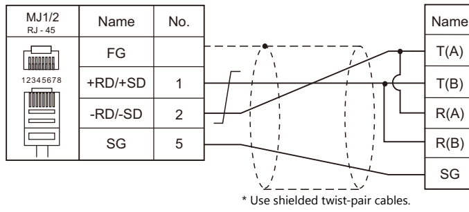
Wiring diagram 3 - M4
