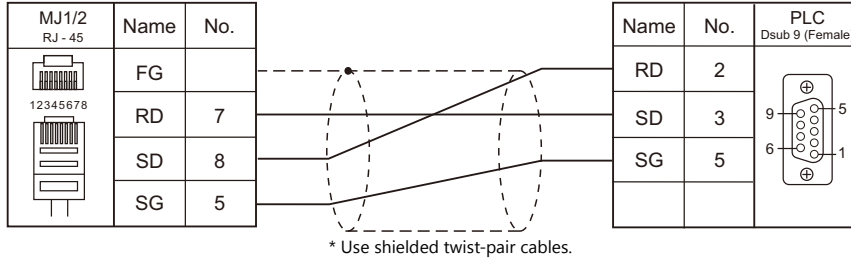
Wiring diagram 2 - M2
