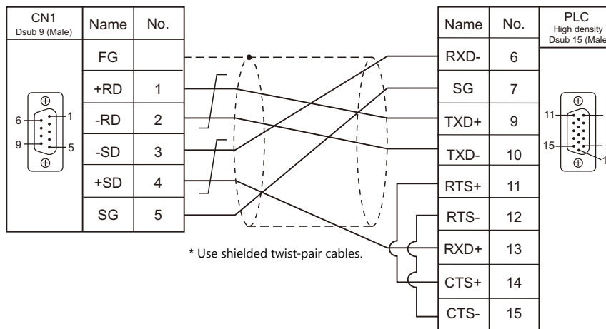
Wiring diagram 3 - C4
