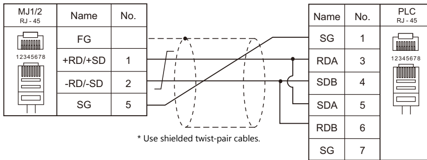
Wiring diagram 1 - M4
