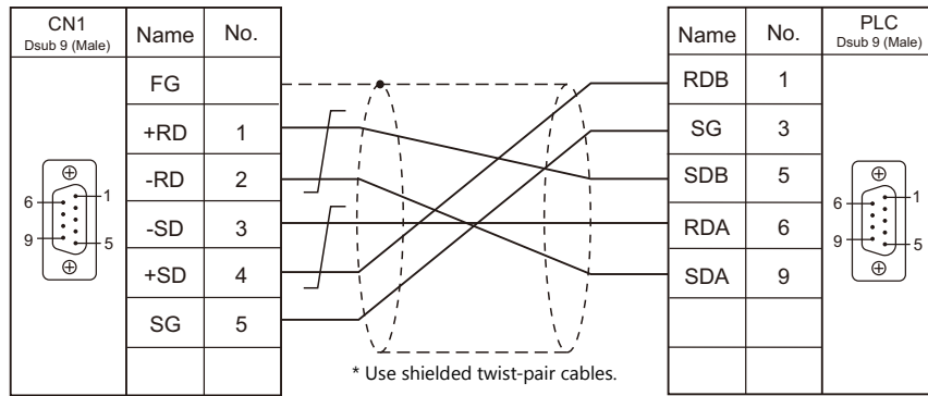
Wiring diagram 2 - C4
