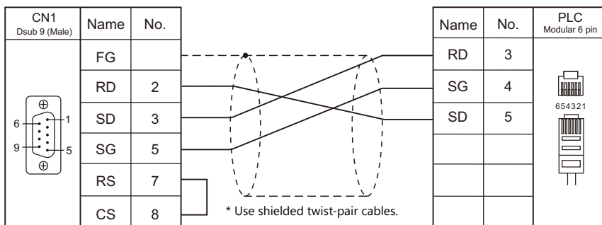
Wiring diagram 3 - C2
