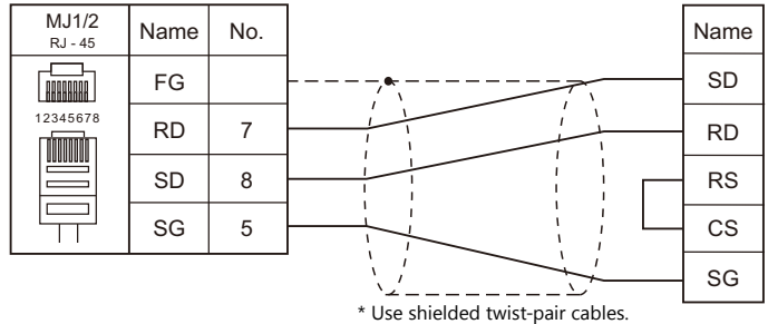
Wiring diagram 4 - M2
