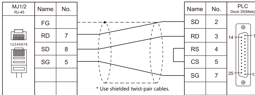
Wiring diagram 2 - M2
