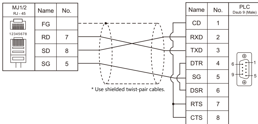
Wiring diagram 2 - M2
