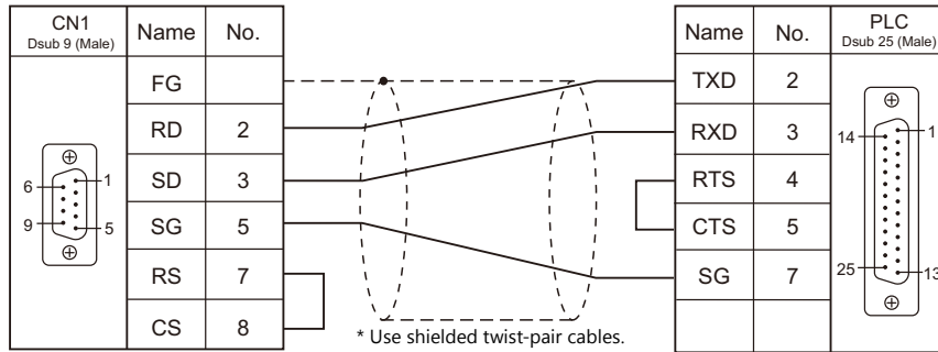
Wiring diagram 2 - C2
