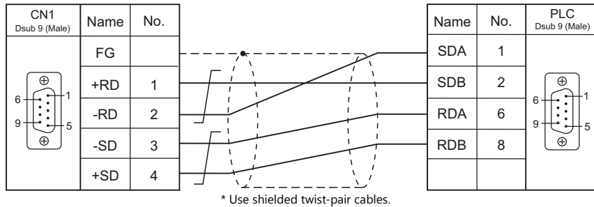
Wiring diagram 4 - C4
