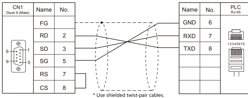
Wiring diagram 3 - C2
