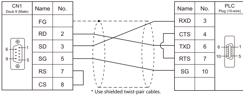
Wiring diagram 6 - C2
