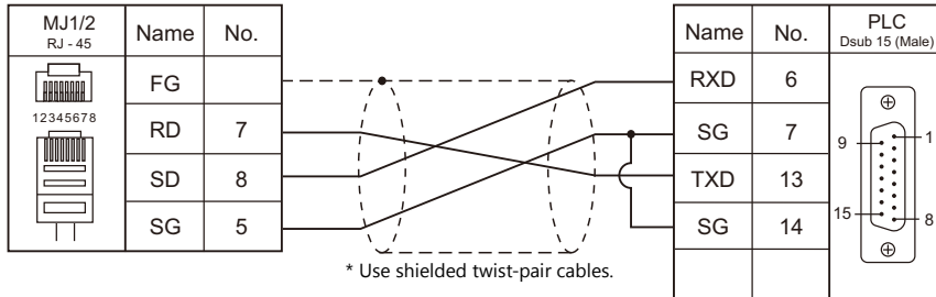
Wiring diagram 4 - M2
