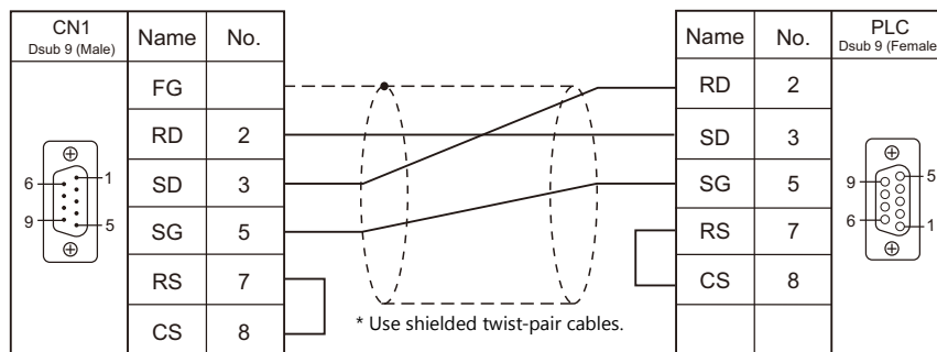
Wiring diagram 4 - C2
