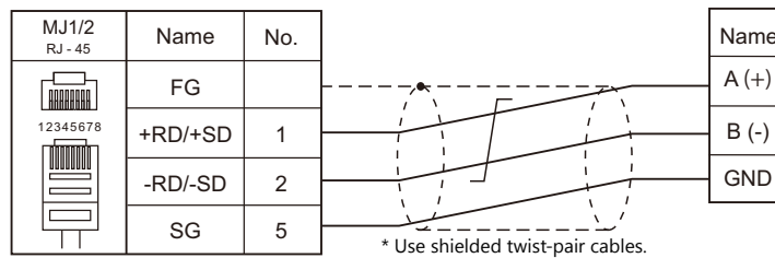
Wiring diagram 1 - M4
