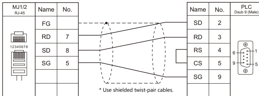
Wiring diagram 3 - M2
