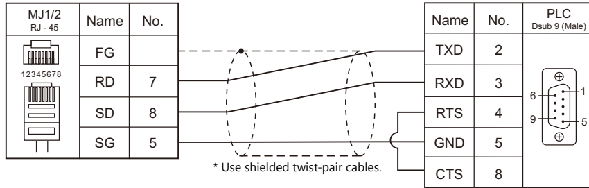
Wiring diagram 3 - M2
