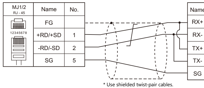
Wiring diagram 2 - M4
