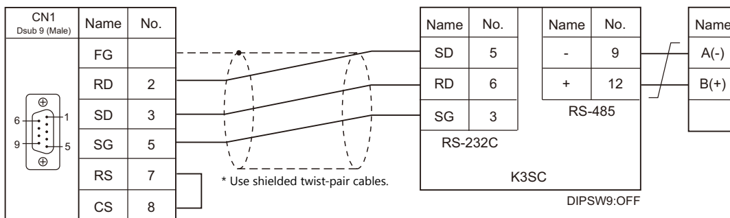
Wiring diagram 4 - C2
