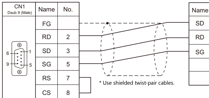
Wiring diagram 2 - C2
