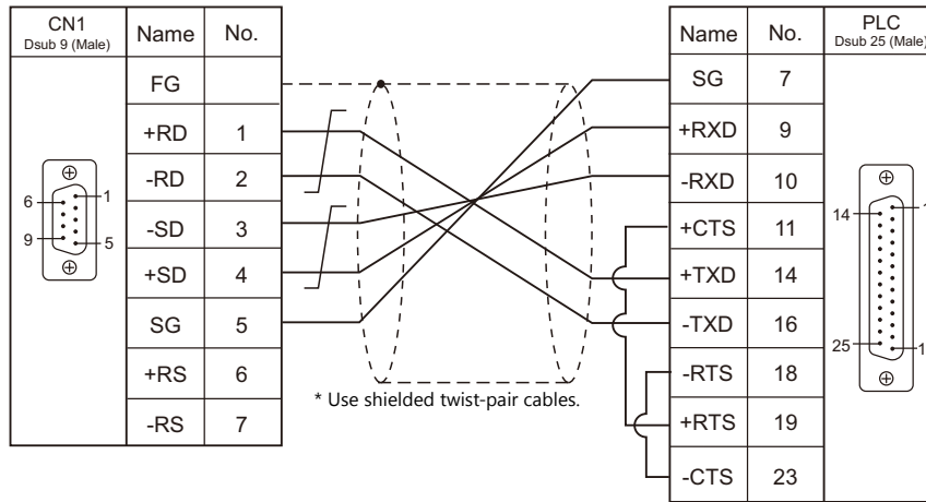
Wiring diagram 2 - C4
