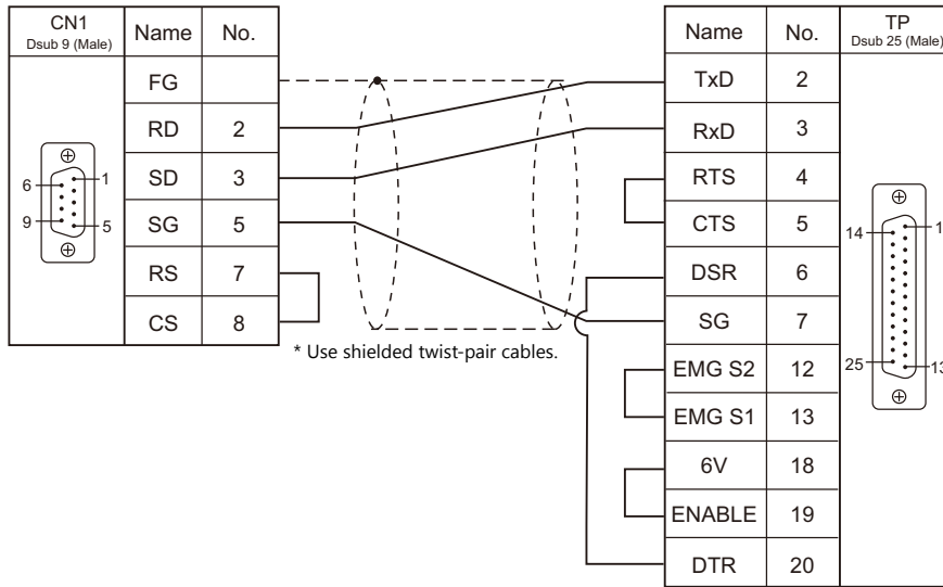
Wiring diagram 3 - C2
