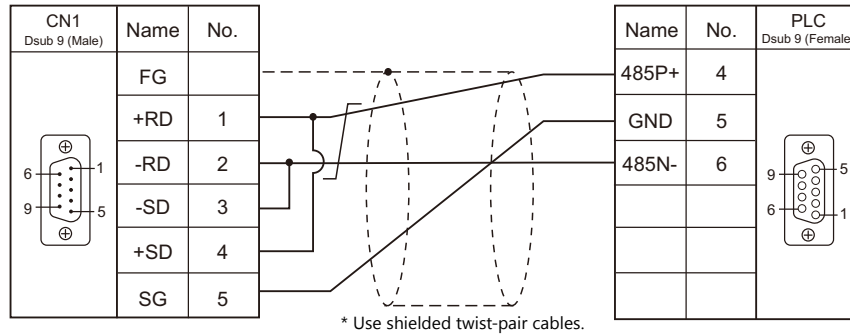
Wiring diagram 5 - C4
