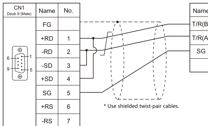
Wiring diagram 1 - C4
