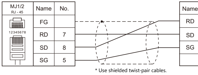
Wiring diagram 2 - M2
