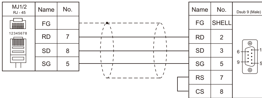
Wiring diagram 6 - M2
