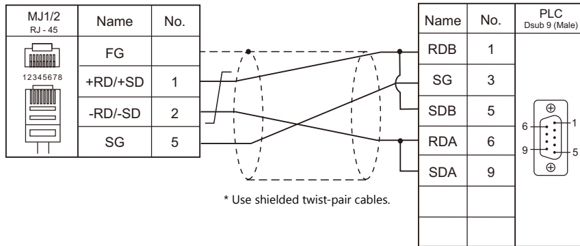
Wiring diagram 5 - M4
