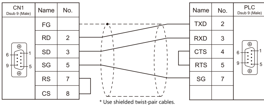
Wiring diagram 7 - C2
