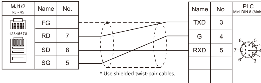
Wiring diagram 3 - M2
