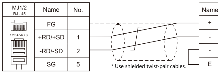
Wiring diagram 2 - M4
