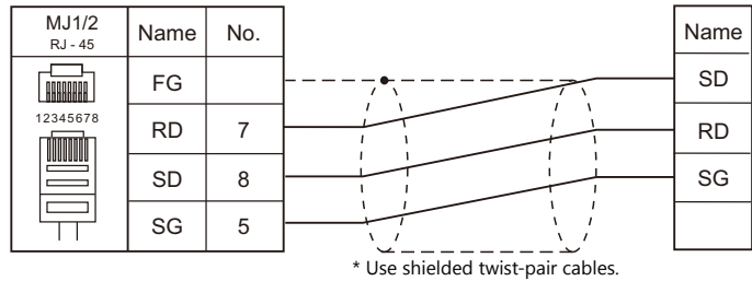
Wiring diagram 3 - M2
