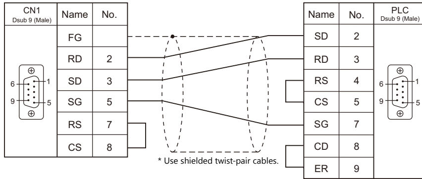
Wiring diagram 2 - C2
