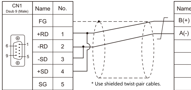
Wiring diagram 2 - C4
