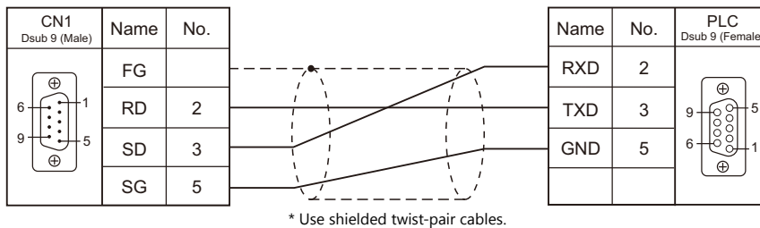
Wiring diagram 1 - C2
