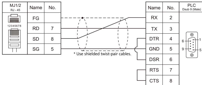
Wiring diagram 1 - M2
