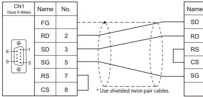
Wiring diagram 4 - C2
