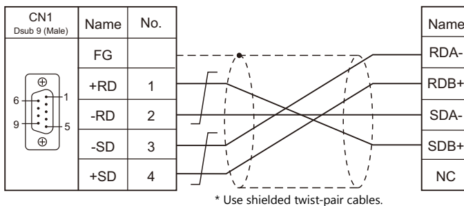
Wiring diagram 4 - C4
