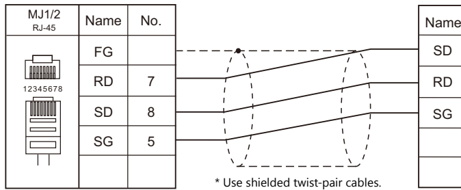
Wiring diagram 1 - M2
