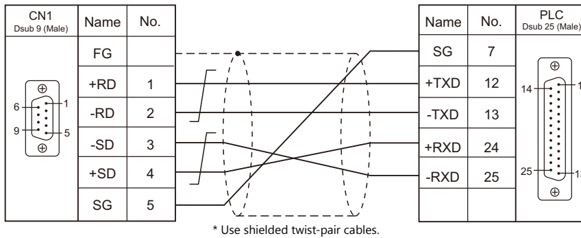
Wiring diagram 2 - C4
