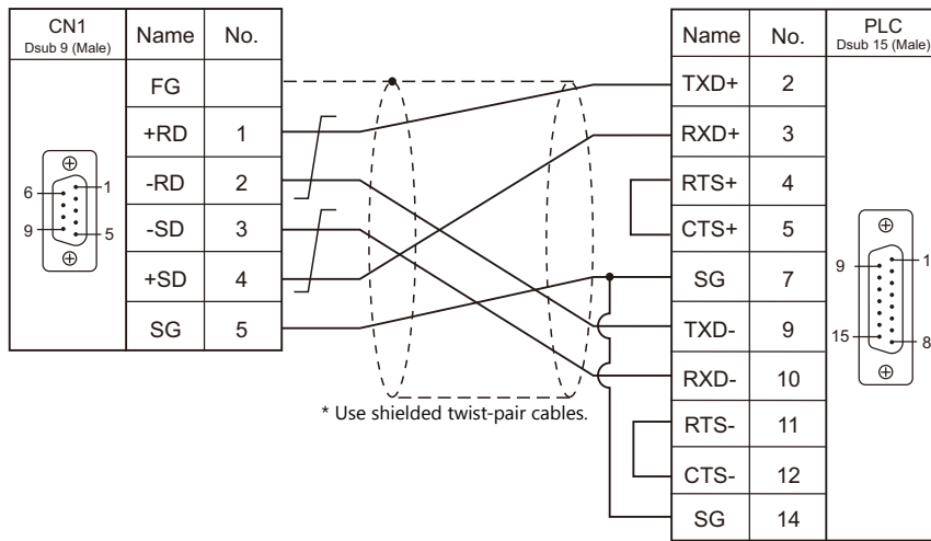
Wiring diagram 4 - C4
