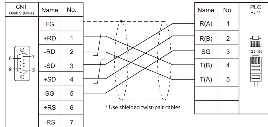
Wiring diagram 2 - C4
