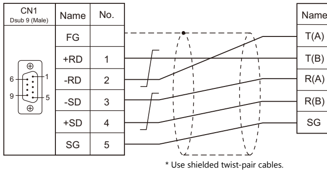
Wiring diagram 3 - C4
