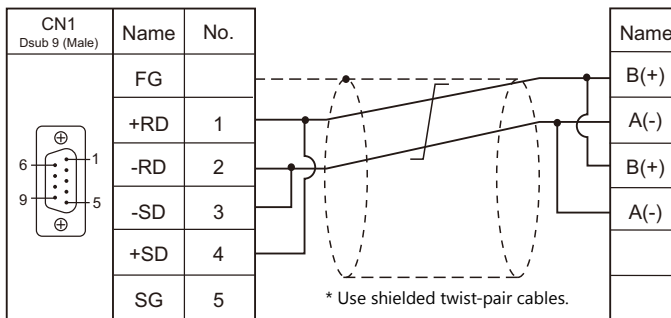
Wiring diagram 4 - C4
