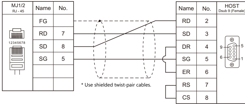
Wiring diagram 2 - M2
