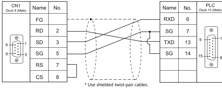
Wiring diagram 4 - C2
