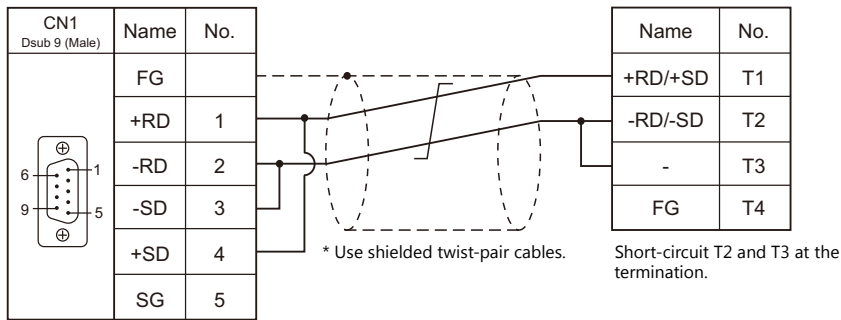
Wiring diagram 1 - C4
