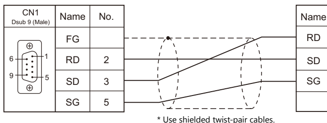
Wiring diagram 2 - C2
