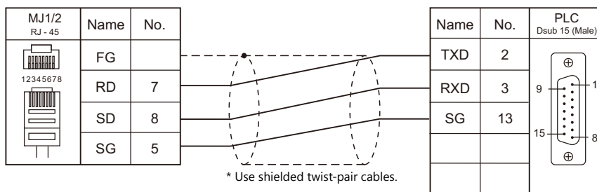
Wiring diagram 4 - M2
