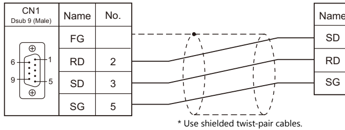
Wiring diagram 1 - C2
