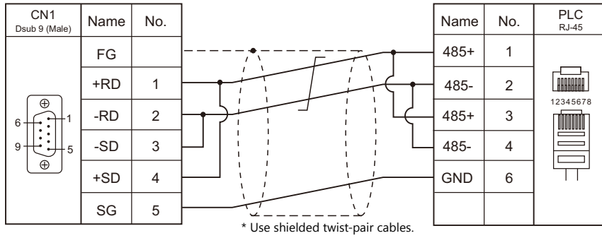
Wiring diagram 3 - C4
