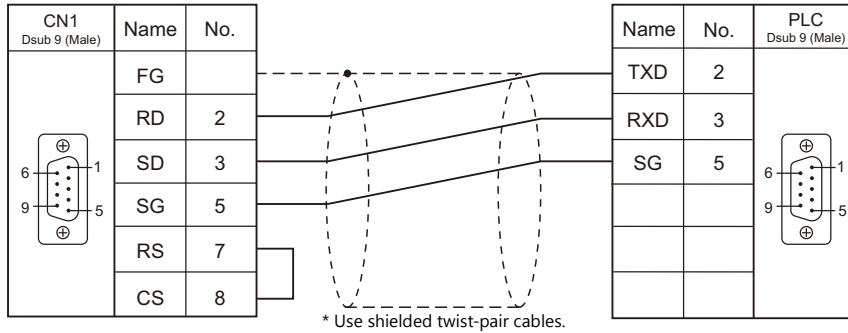
Wiring diagram 1 - C2
