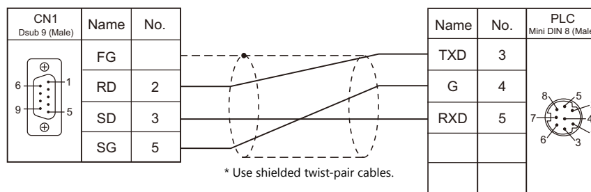
Wiring diagram 3 - C2
