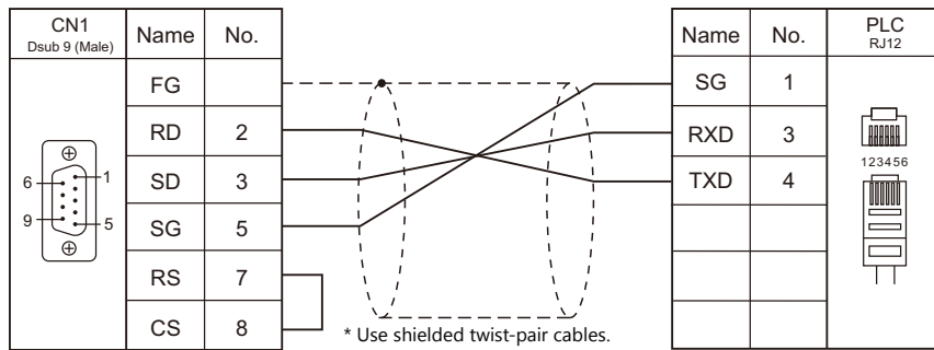
Wiring diagram 3 - C2
