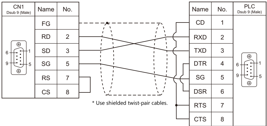
Wiring diagram 2 - C2
