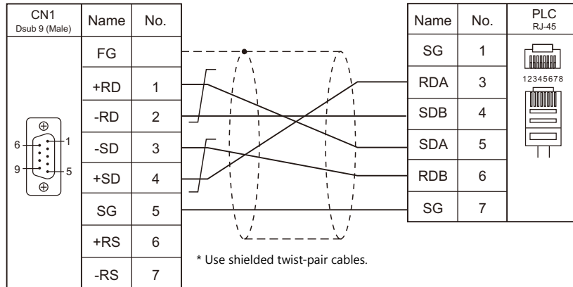
Wiring diagram 2 - C4
