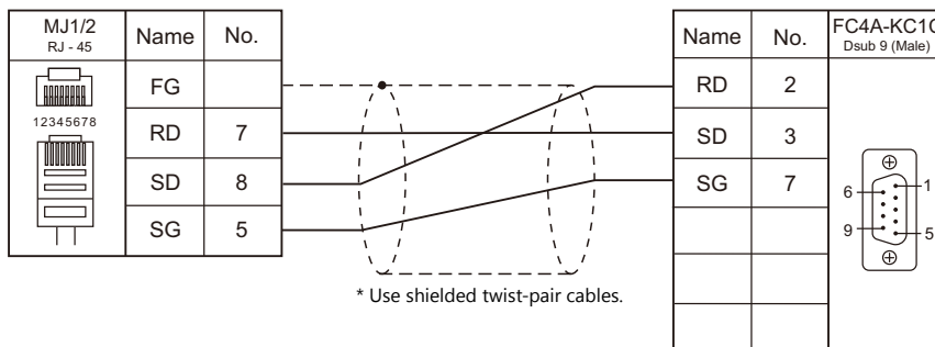
Wiring diagram 4 - M2
