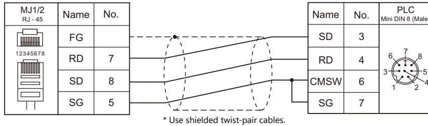
Wiring diagram 3 - M2
