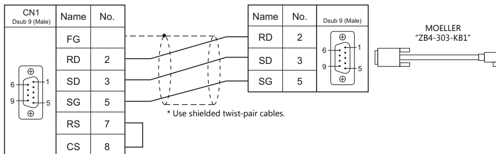
Wiring diagram 2 - C2
