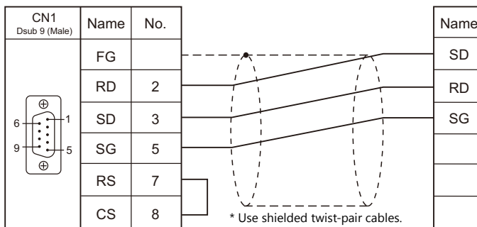
Wiring diagram 3 - C2
