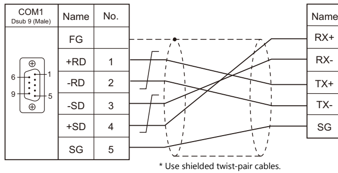
Wiring diagram 2 - C4
