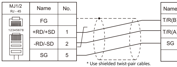
Wiring diagram 2 - M4
