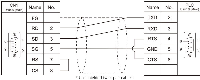
Wiring diagram 2 - C2
