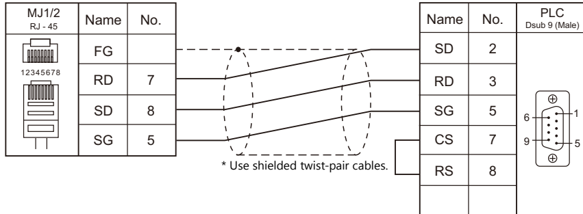
Wiring diagram 1 - M2
