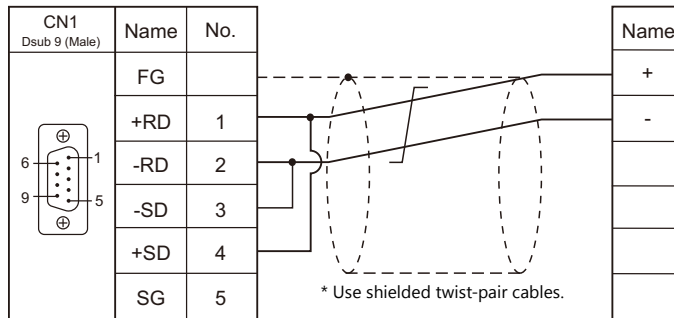
Wiring diagram 1 - C4
