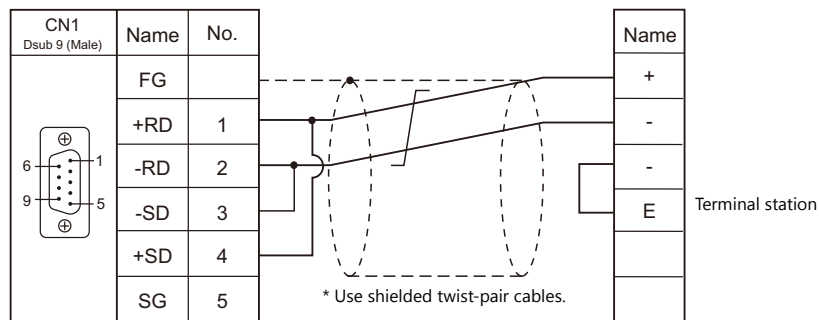
Wiring diagram 2 - C4
