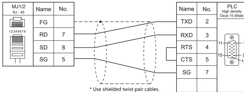
Wiring diagram 3 - M2
