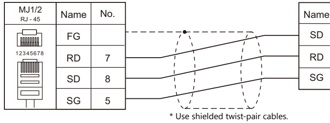
Wiring diagram 1 - M2
