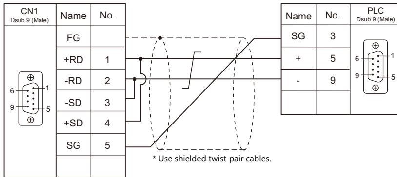
Wiring diagram 5 - C4
