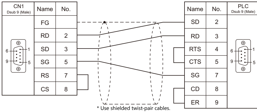
Wiring diagram 5 - C2
