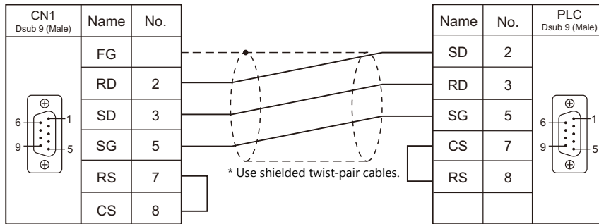
Wiring diagram 1 - C2
