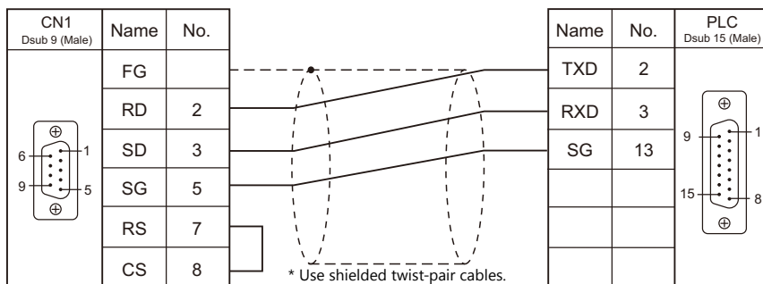
Wiring diagram 4 - C2
